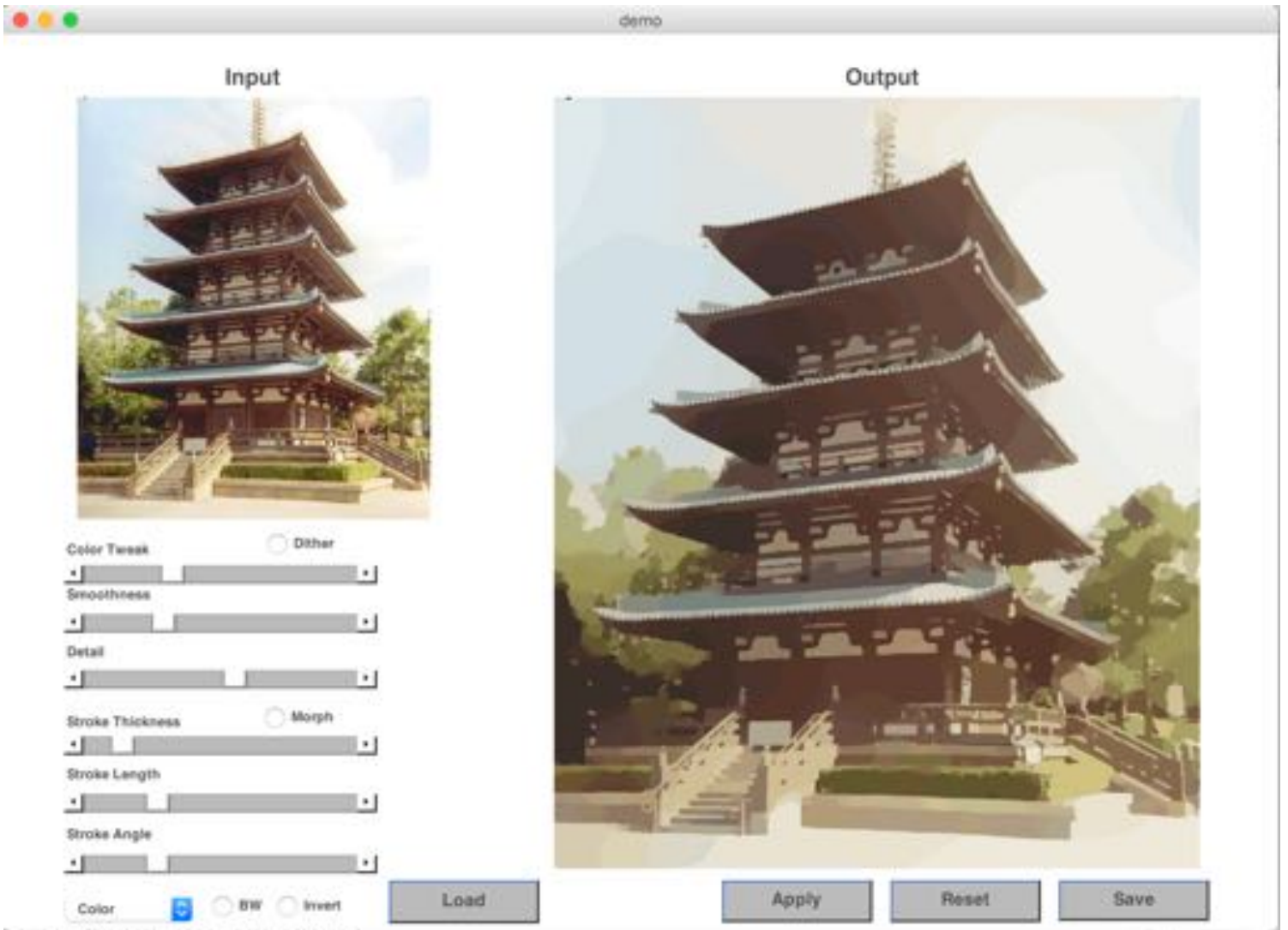
Figure 8: GUI Instance
