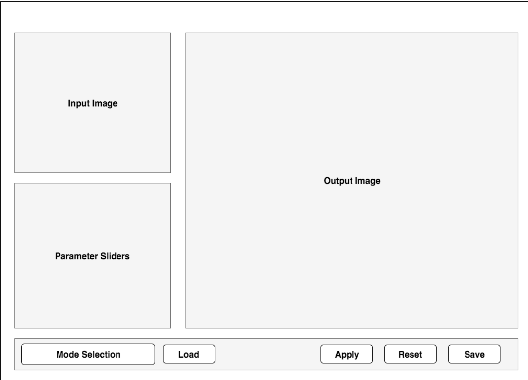
Figure 1: GUI Wireframe
